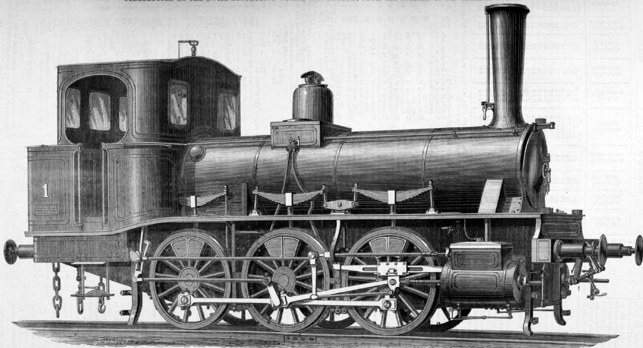
TANK LOCOMOTIVE FOR BRANCH RAILWAYS. CONSTRUCTED AT THE SWISS LOCOMOTIVE WORKS, WINTERTHUR; FROM THE DESIGNS OF MR. CHARLES BROWN.
