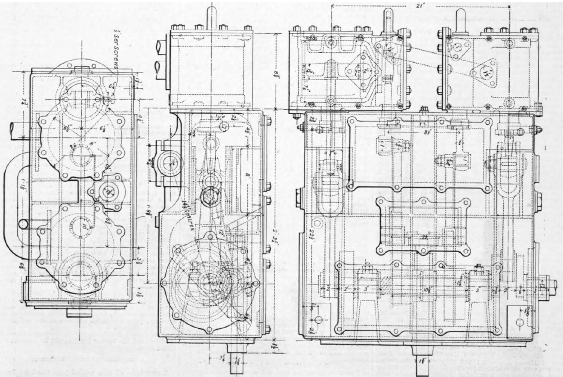
COMPOUND STEAM ENGINE FOR MOTOR WAGON
